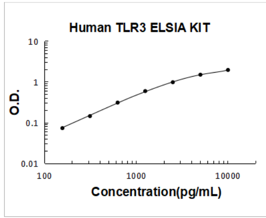
Human TLR3 PicoKine ELISA Kit standard curve
