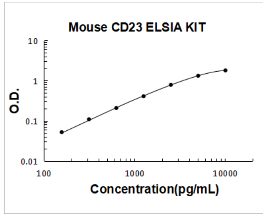
Mouse CD23/FCER2 PicoKine ELISA Kit standard curve
