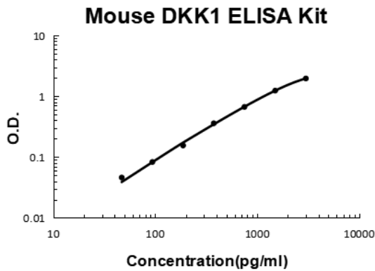
Mouse DKK1 PicoKine ELISA Kit standard curve
