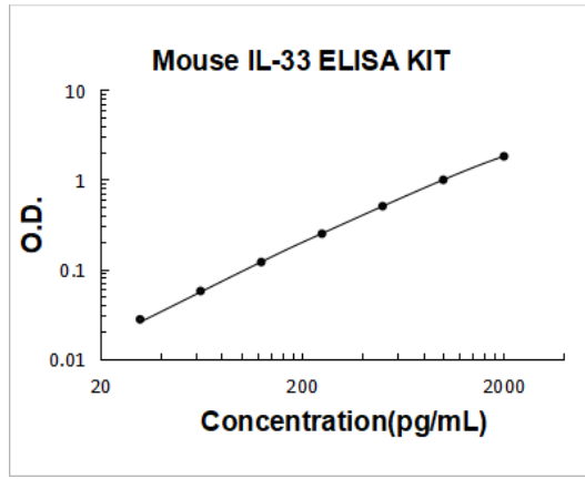
Mouse IL-33 PicoKine ELISA Kit standard curve
