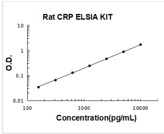
Rat CRP PicoKine ELISA Kit standard curve
