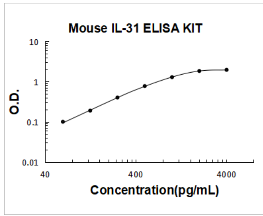
Mouse IL-31 PicoKine ELISA Kit standard curve
