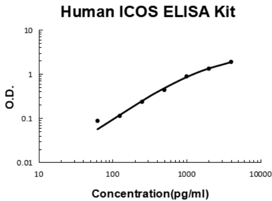
Human ICOS PicoKine ELISA Kit standard curve
