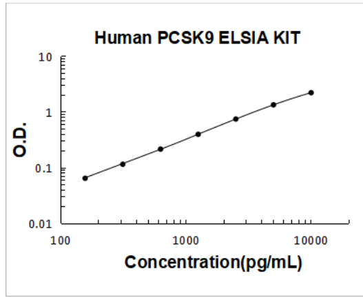
Human PCSK9 PicoKine ELISA Kit standard curve
