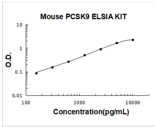
Mouse PCSK9 PicoKine ELISA Kit standard curve
