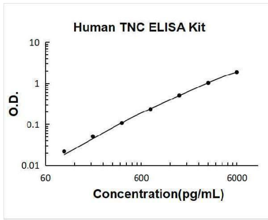
Human Tenascin-C PicoKine ELISA Kit standard curve
