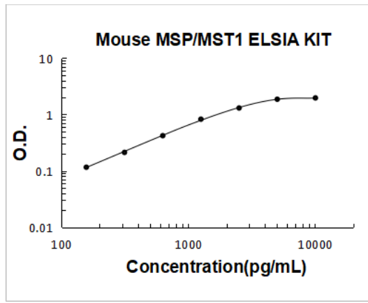
Mouse MSP/MST1 PicoKine ELISA Kit standard curve
