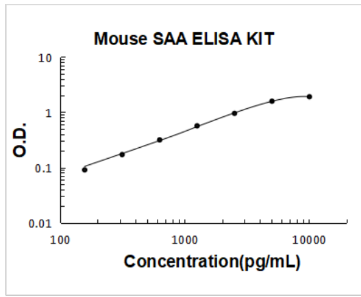
Mouse SAA PicoKine ELISA Kit standard curve
