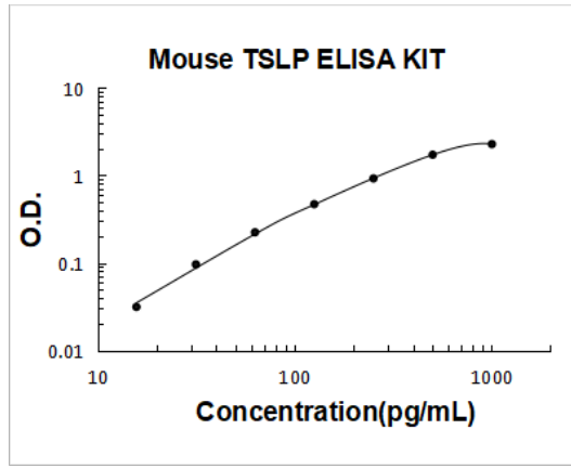
Mouse TSLP PicoKine ELISA Kit standard curve
