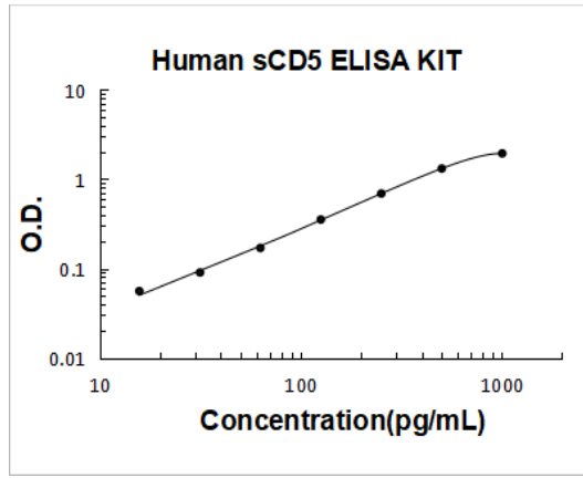
Human soluble CD5 PicoKine ELISA Kit standard curve
