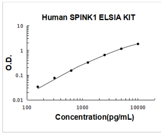
Human SPINK1/TATI PicoKine ELISA Kit standard curve
