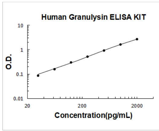
Human Granulysin PicoKine ELISA Kit standard curve
