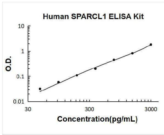
Human SPARCL1 PicoKine ELISA Kit standard curve
