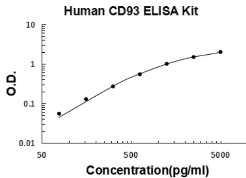
Human CD93/C1qR PicoKine ELISA Kit standard curve
