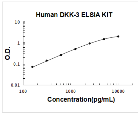
Human DKK-3 PicoKine ELISA Kit standard curve
