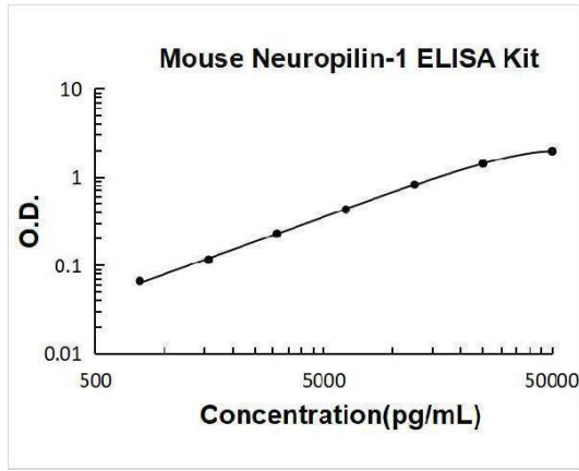
Mouse Neuropilin-1 PicoKine ELISA Kit standard curve
