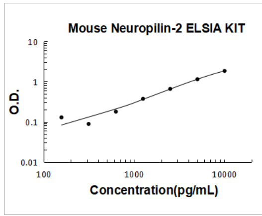
Mouse Neuropilin-2 PicoKine ELISA Kit standard curve
