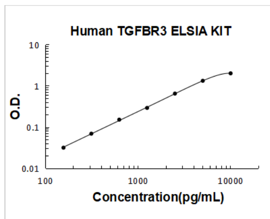
Human TGFBR3 PicoKine ELISA Kit standard curve
