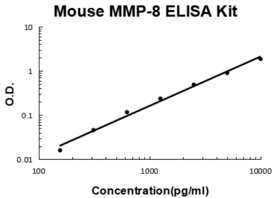
Mouse MMP-8 PicoKine ELISA Kit standard curve
