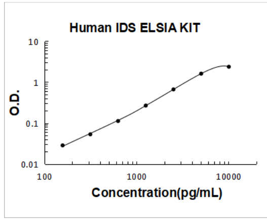
Human IDS PicoKine ELISA Kit standard curve
