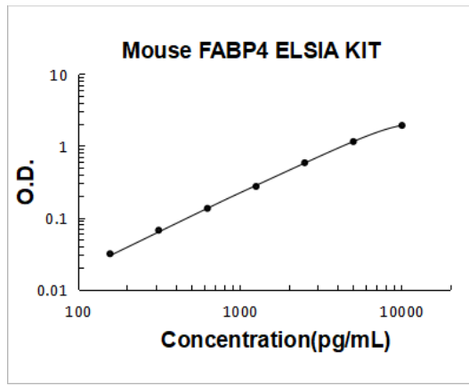
Mouse FABP4 PicoKine ELISA Kit standard curve
