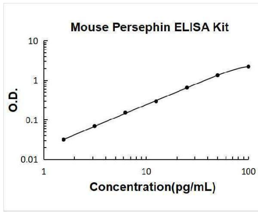
Mouse Persephin PicoKine ELISA Kit standard curve
