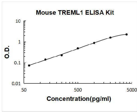
Mouse TREML1 PicoKine ELISA Kit standard curve
