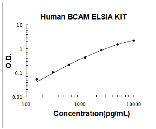
Human BCAM PicoKine ELISA Kit standard curve
