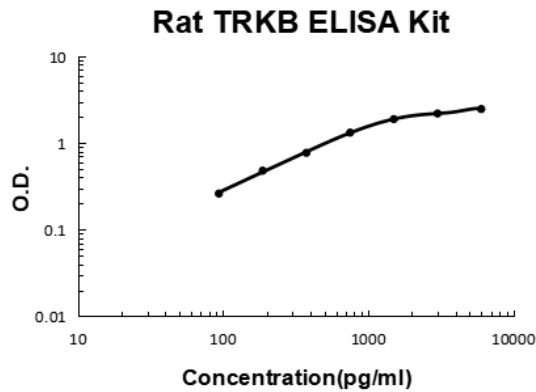
Rat TRKB PicoKine ELISA Kit standard curve
