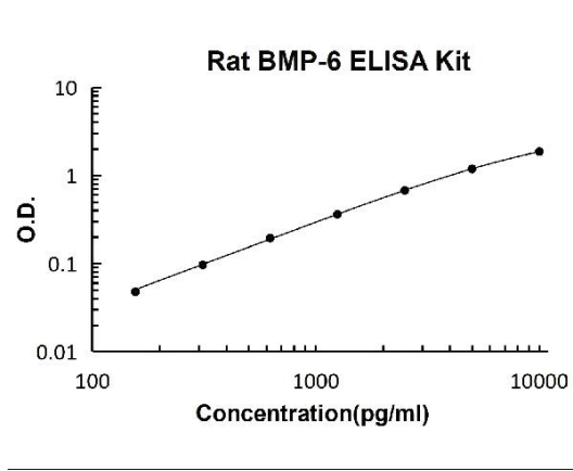
Rat BMP-6 PicoKine ELISA Kit standard curve
