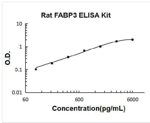
Rat FABP3 PicoKine ELISA Kit standard curve
