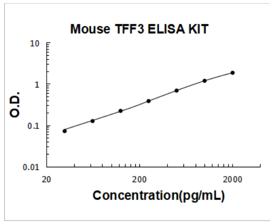
Mouse TFF3 PicoKine ELISA Kit standard curve
