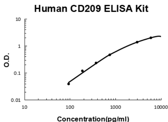
Human CD209 PicoKine ELISA Kit standard curve
