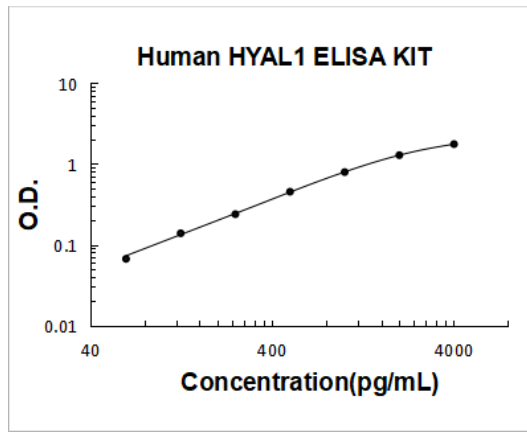
Human HYAL1 PicoKine ELISA Kit standard curve
