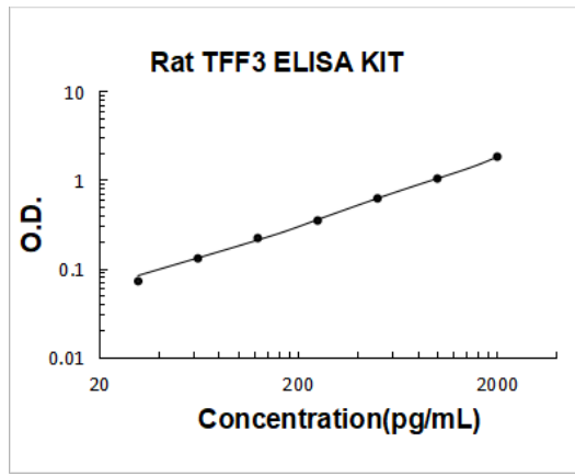
Rat TFF3 PicoKine ELISA Kit standard curve
