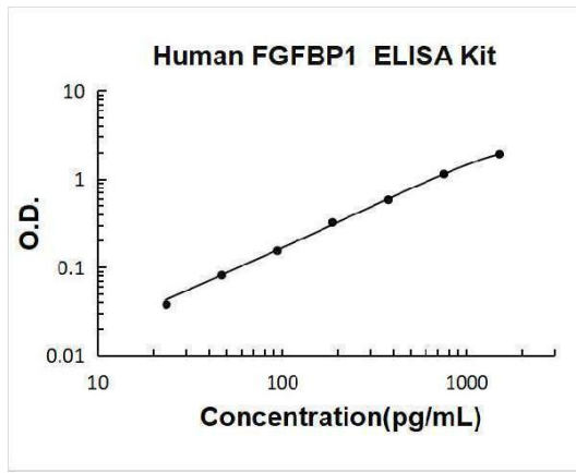
Human FGFBP1 PicoKine ELISA Kit standard curve
