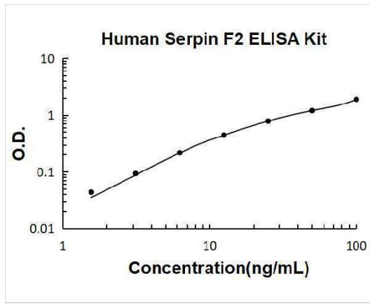
Human SerpinF2 PicoKine ELISA Kit standard curve
