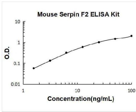
Mouse SerpinF2 PicoKine ELISA Kit standard curve
