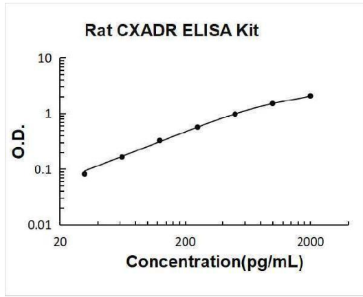
Rat CXADR PicoKine ELISA Kit standard curve
