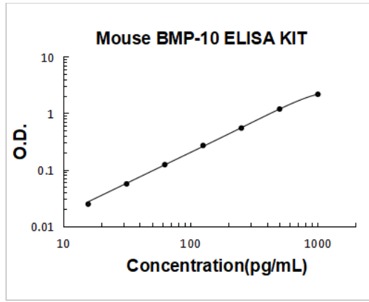
Mouse BMP-10 PicoKine ELISA Kit standard curve
