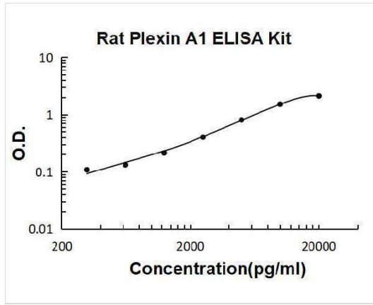
Rat Plexin A1 PicoKine ELISA Kit standard curve
