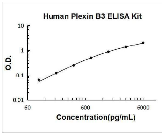
Human Plexin B3 PicoKine ELISA Kit standard curve
