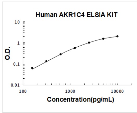
Human AKR1C4 PicoKine ELISA Kit Standard Curve
