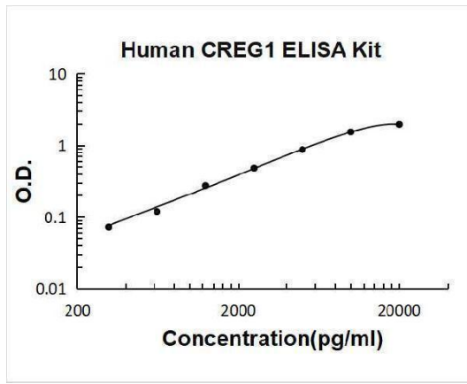
Human CREG1 PicoKine ELISA Kit standard curve
