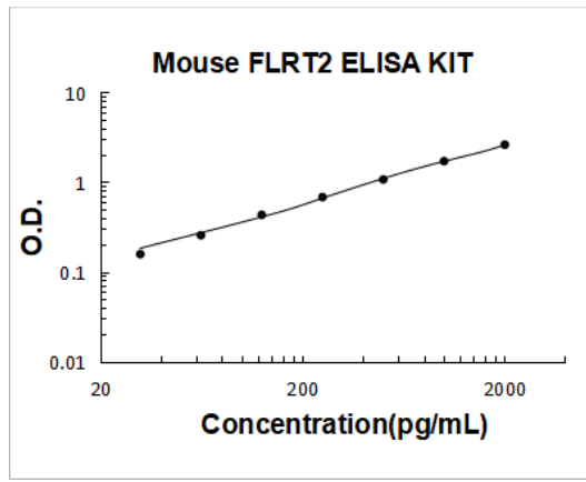
Mouse FLRT2 PicoKine ELISA Kit standard curve
