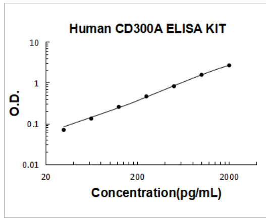
Human CD300A PicoKine ELISA Kit Standard Curve
