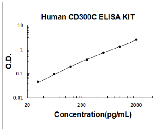
Human CD300C PicoKine ELISA Kit Standard Curve
