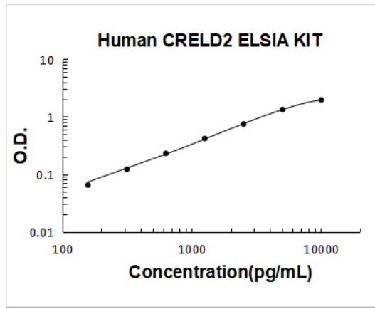
Human CRELD2 PicoKine ELISA Kit Standard Curve
