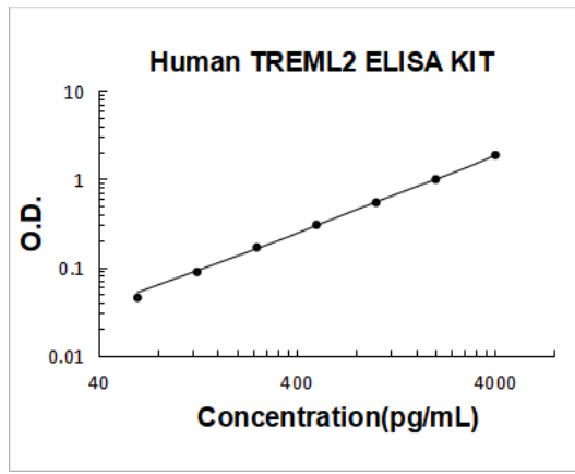
Human TREML2 PicoKine ELISA Kit Standard Curve
