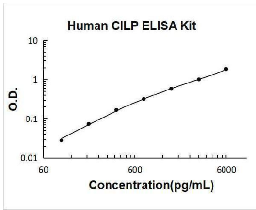
Human CILP PicoKine ELISA Kit Standard Curve
